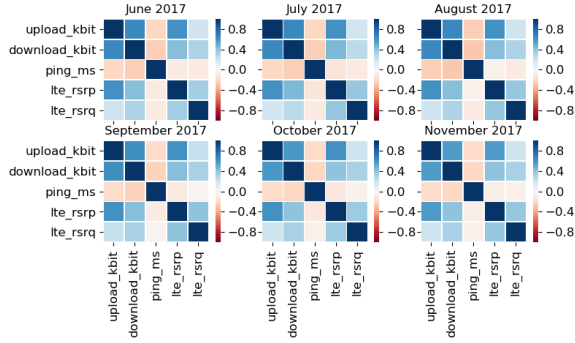
Fig. 4: Pearson's correlations in the RTR Nettetst platform.
