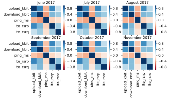
Fig. 6: Spearman's correlations in the RTR Nettetst platform.
