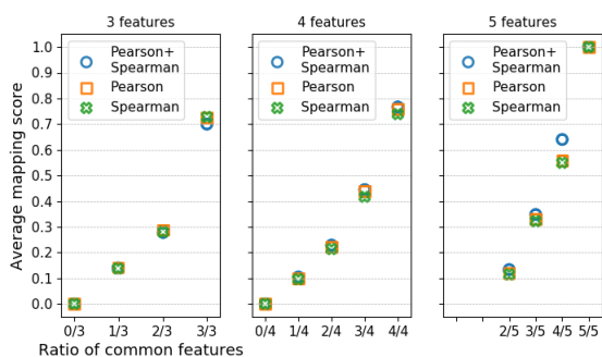
Fig. 7: Average mapping scores when mapping from RTR Nettetst to Netradar. The score increases as a function of the common ratio. The perfect mappings (ratio of 1.0) outperforms the incomplete mappings.
